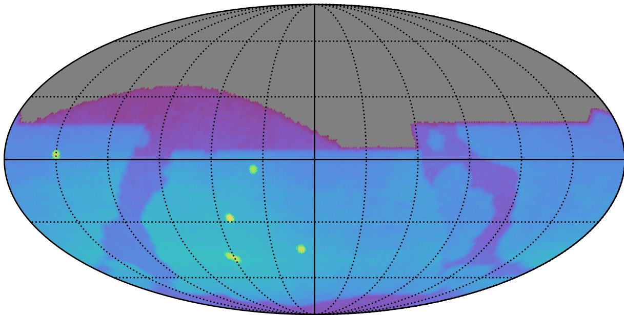
ddf_loaded_half_fl15_v3.4_10yrs : Brown Dwarf, L7
