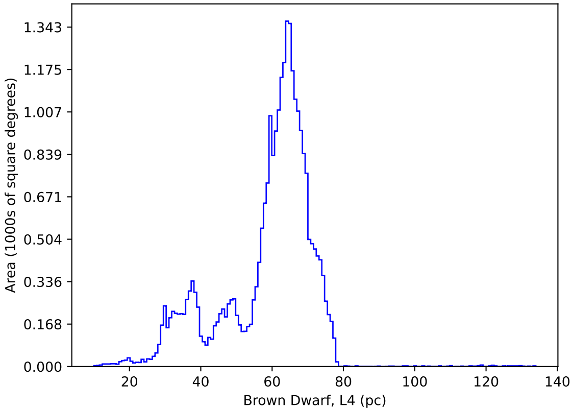
ddf_loaded_half_fl15_v3.4_10yrs : Brown Dwarf, L4
