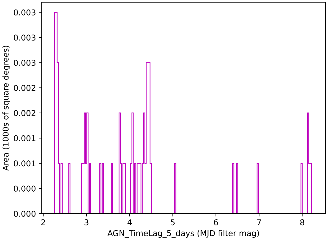
ddf_loaded_half_fl15_v3.4_10yrs z band: AGN_TimeLag_5_days
