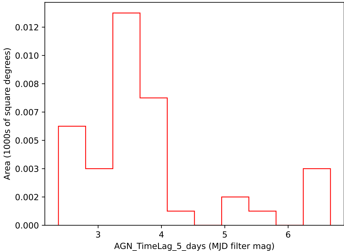
ddf_loaded_half_fl15_v3.4_10yrs i band: AGN_TimeLag_5_days
