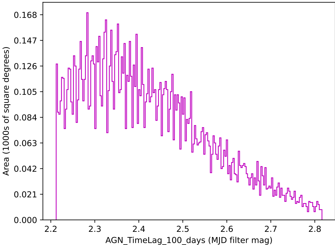
ddf_loaded_half_fl15_v3.4_10yrs z band: AGN_TimeLag_100_days
