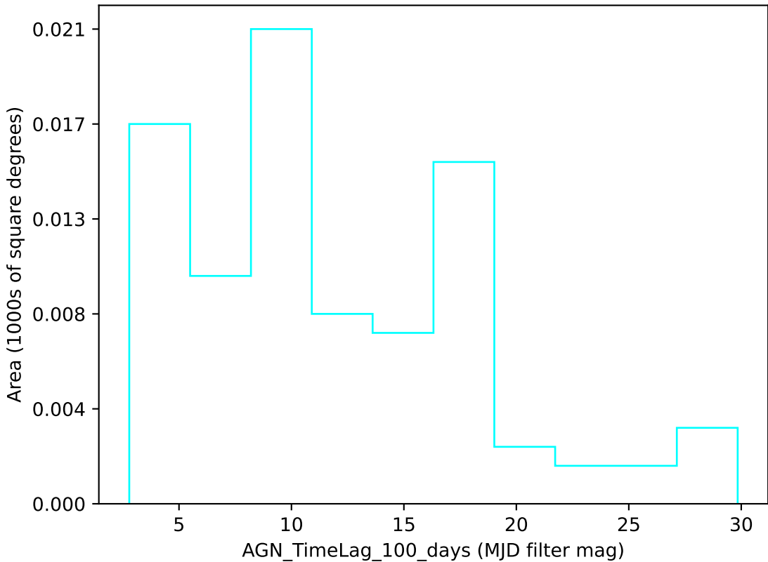
ddf_loaded_half_fl15_v3.4_10yrs u band: AGN_TimeLag_100_days
