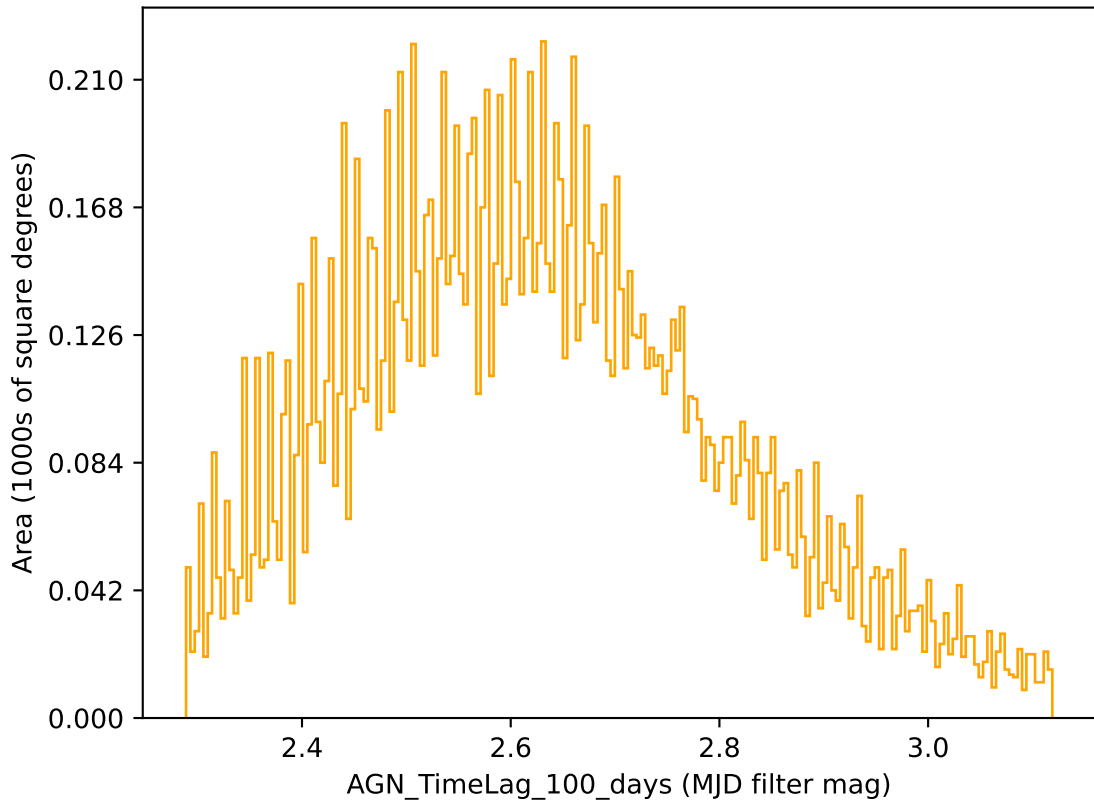
ddf_loaded_half_fl15_v3.4_10yrs r band: AGN_TimeLag_100_days
