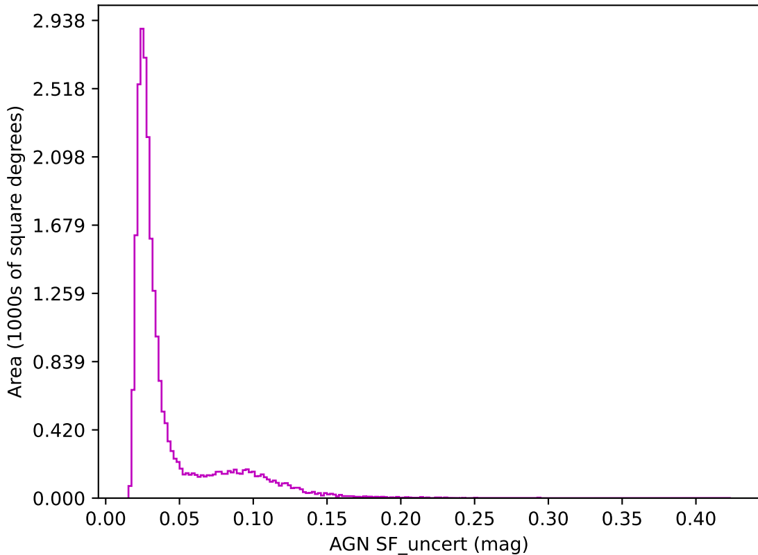
ddf_loaded_half_fl15_v3.4_10yrs z band: AGN SF_uncert
