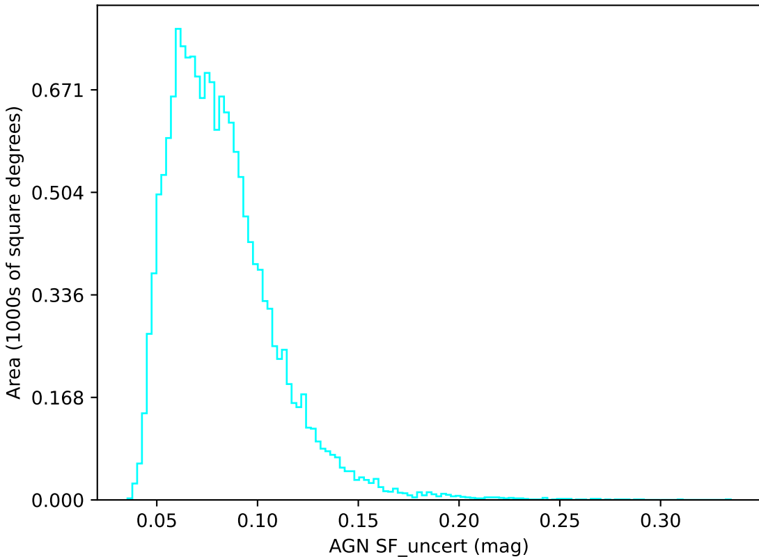
ddf_loaded_half_fl15_v3.4_10yrs u band: AGN SF_uncert
