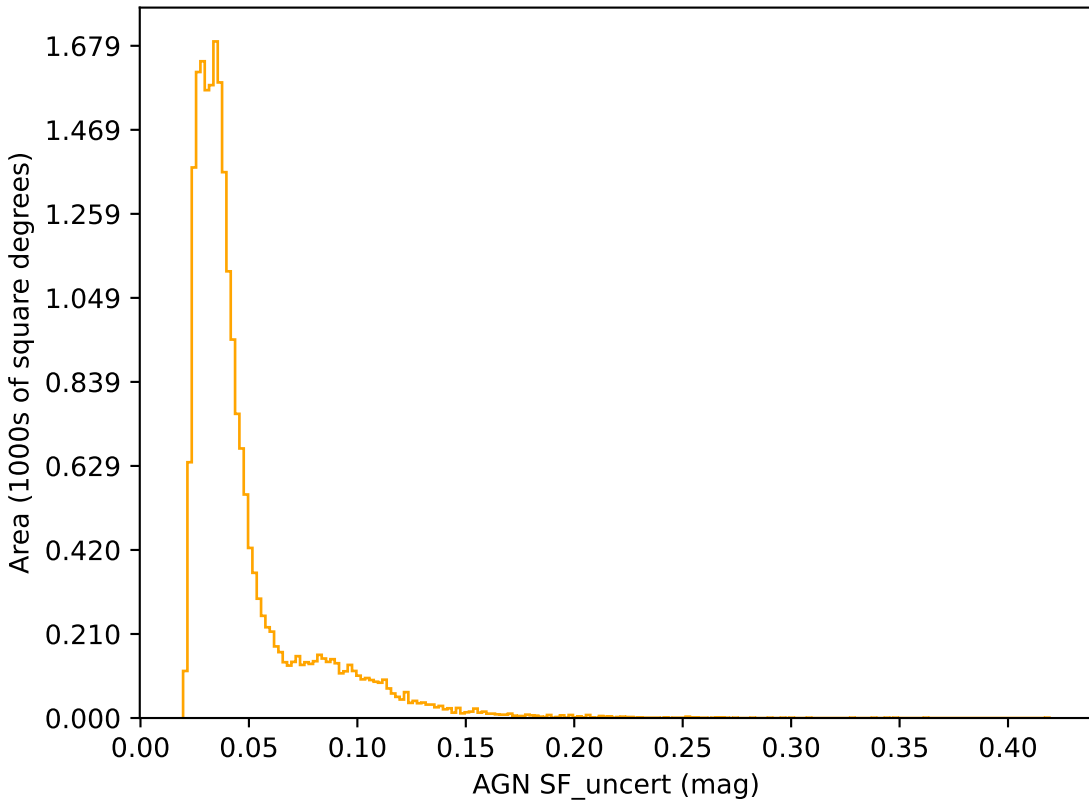
ddf_loaded_half_fl15_v3.4_10yrs r band: AGN SF_uncert
