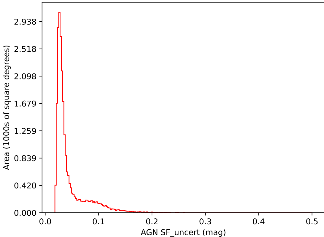
ddf_loaded_half_fl15_v3.4_10yrs i band: AGN SF_uncert
