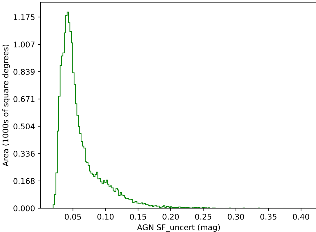
ddf_loaded_half_fl15_v3.4_10yrs g band: AGN SF_uncert
