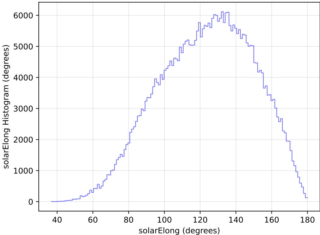
ddf_loaded_half_fl15_v3.4_10yrs WFD y band: solarElong Histogram
