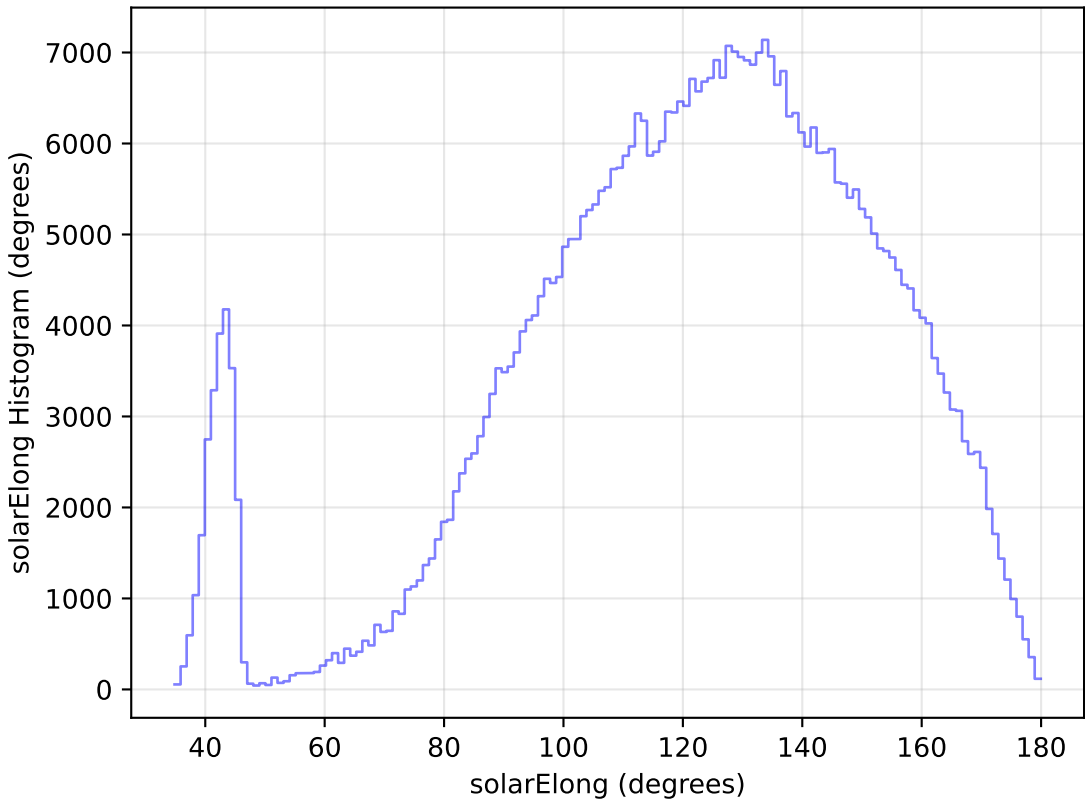
ddf_loaded_half_fl15_v3.4_10yrs WFD i band: solarElong Histogram
