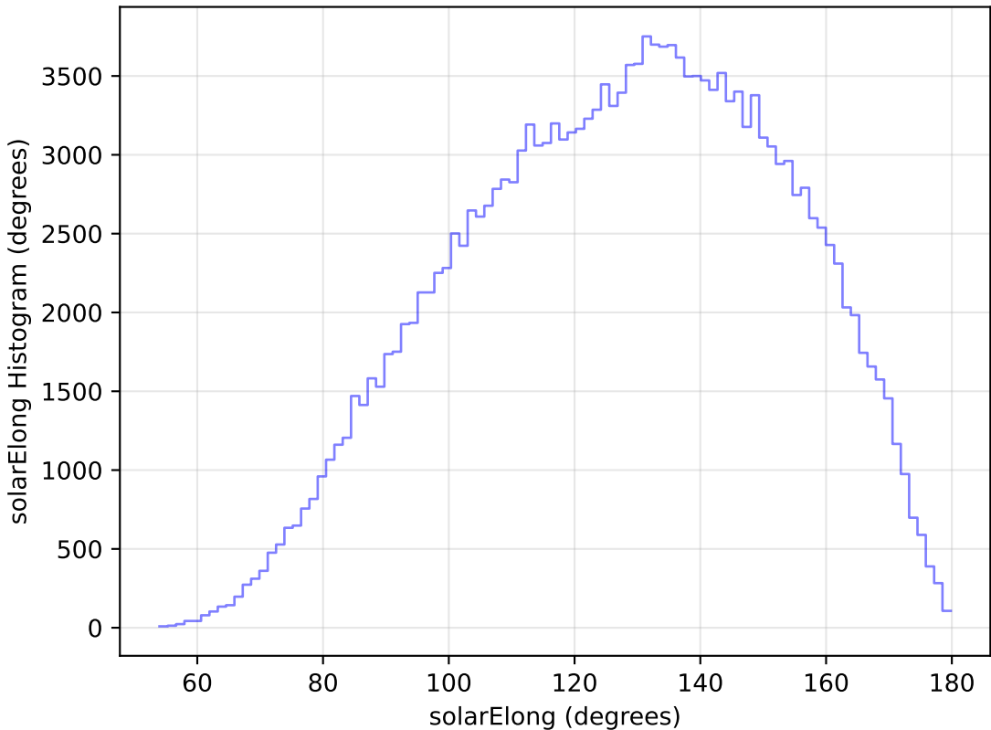
ddf_loaded_half_fl15_v3.4_10yrs WFD g band: solarElong Histogram
