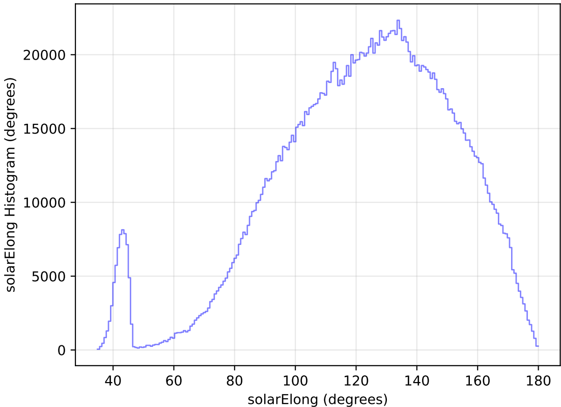
ddf_loaded_half_fl15_v3.4_10yrs WFD all bands: solarElong Histogram
