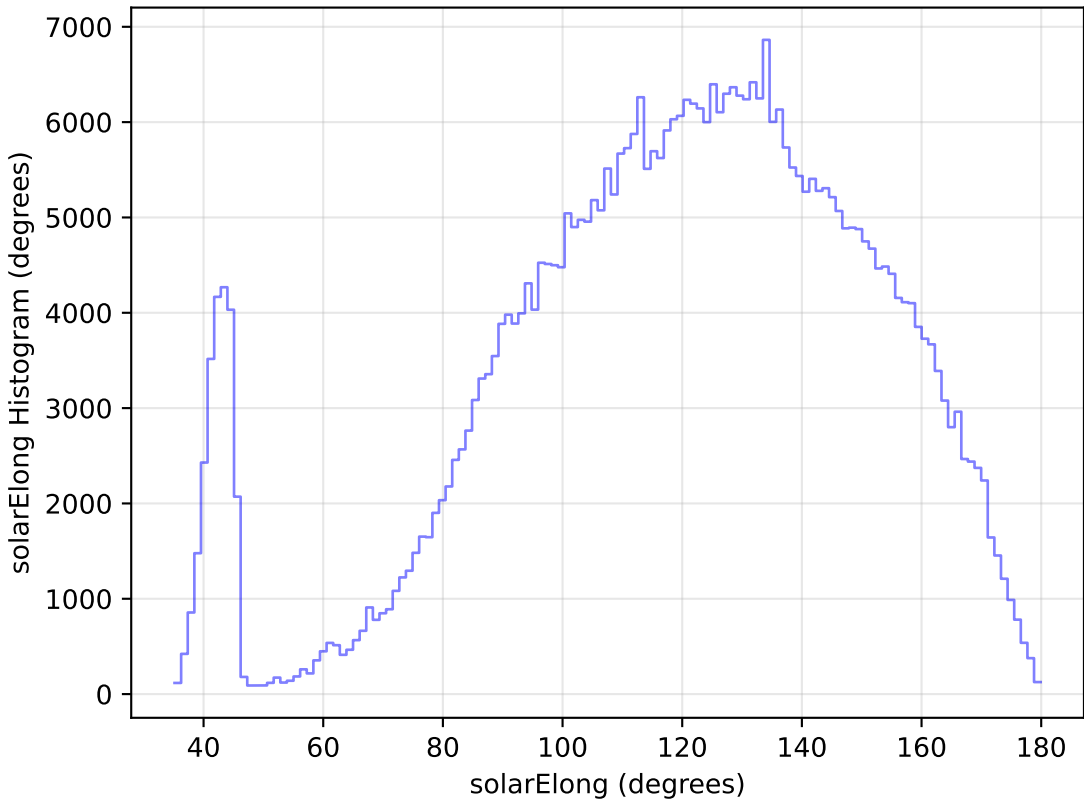
ddf_loaded_half_fl15_v3.4_10yrs All sky z band: solarElong Histogram
