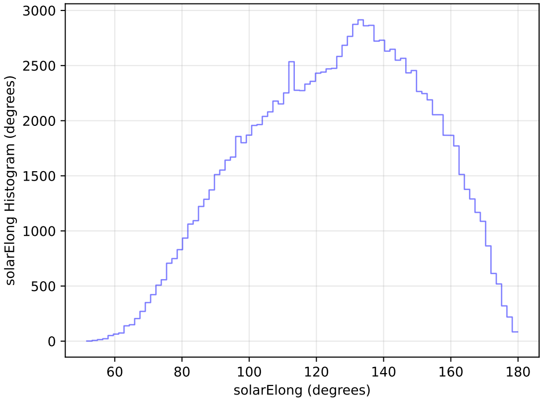
ddf_loaded_half_fl15_v3.4_10yrs All sky u band: solarElong Histogram
