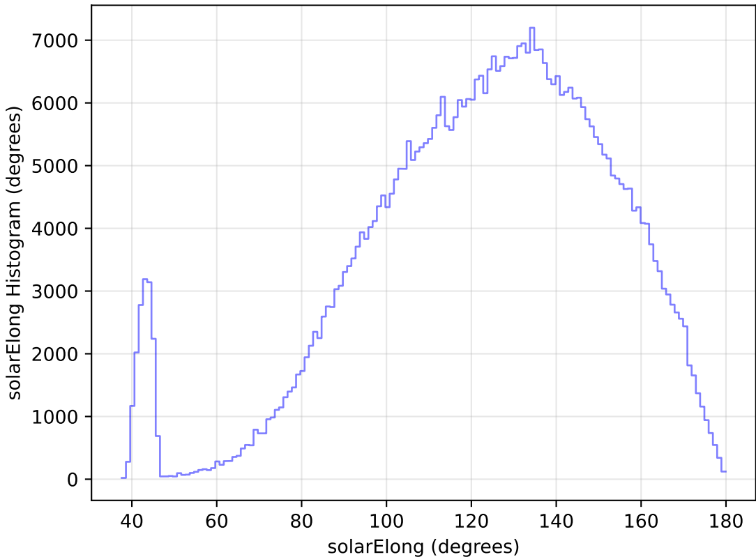
ddf_loaded_half_fl15_v3.4_10yrs All sky r band: solarElong Histogram
