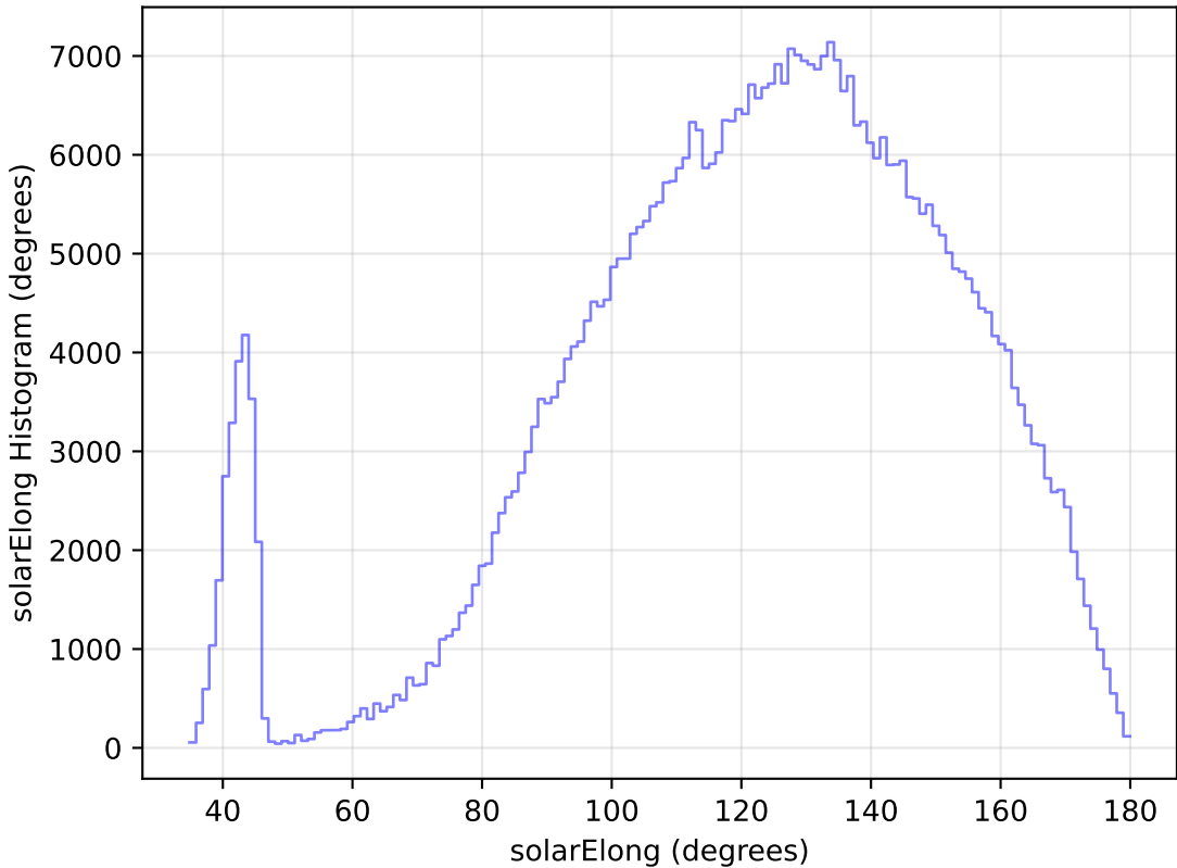
ddf_loaded_half_fl15_v3.4_10yrs All sky i band: solarElong Histogram
