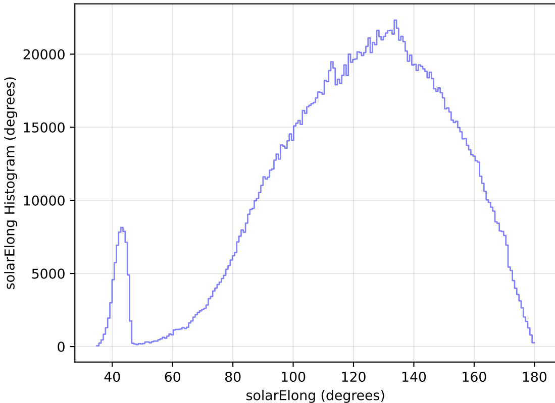
ddf_loaded_half_fl15_v3.4_10yrs All sky all bands: solarElong Histogram
