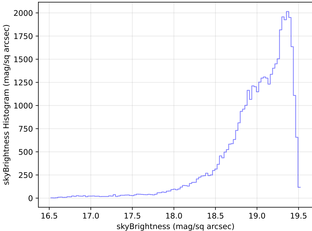
ddf_loaded_half_fl15_v3.4_10yrs Yr 1 z band: skyBrightness Histogram
