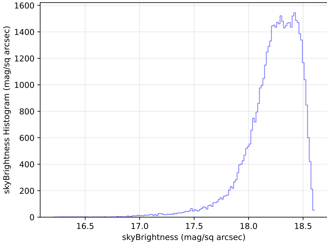
ddf_loaded_half_fl15_v3.4_10yrs Yr 1 y band: skyBrightness Histogram
