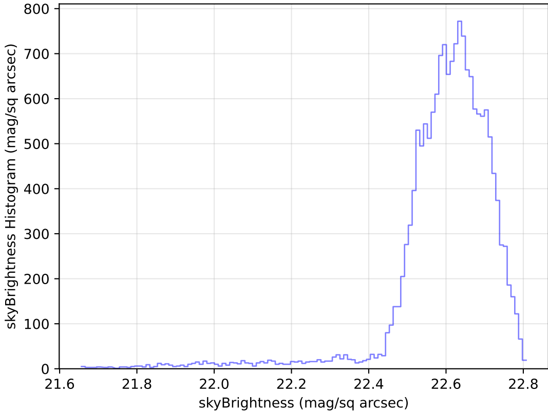
ddf_loaded_half_fl15_v3.4_10yrs Yr 1 u band: skyBrightness Histogram
