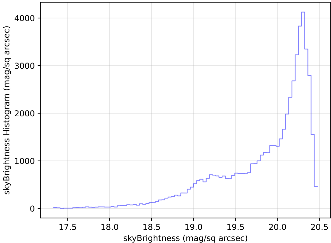
ddf_loaded_half_fl15_v3.4_10yrs Yr 1 i band: skyBrightness Histogram
