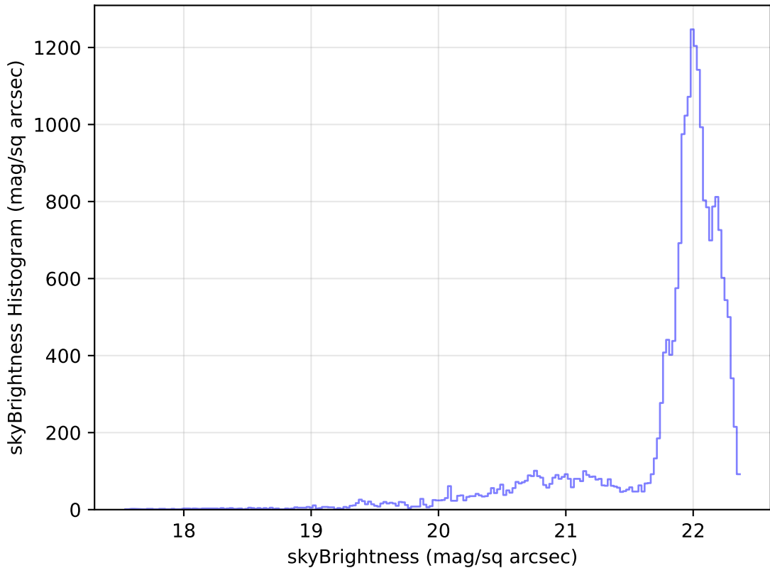
ddf_loaded_half_fl15_v3.4_10yrs Yr 1 g band: skyBrightness Histogram
