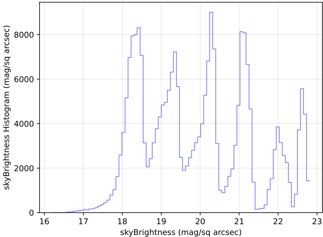
ddf_loaded_half_fl15_v3.4_10yrs Yr 1 all bands: skyBrightness Histogram
