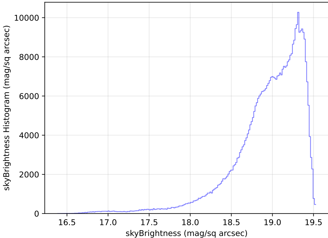
ddf_loaded_half_fl15_v3.4_10yrs WFD z band: skyBrightness Histogram
