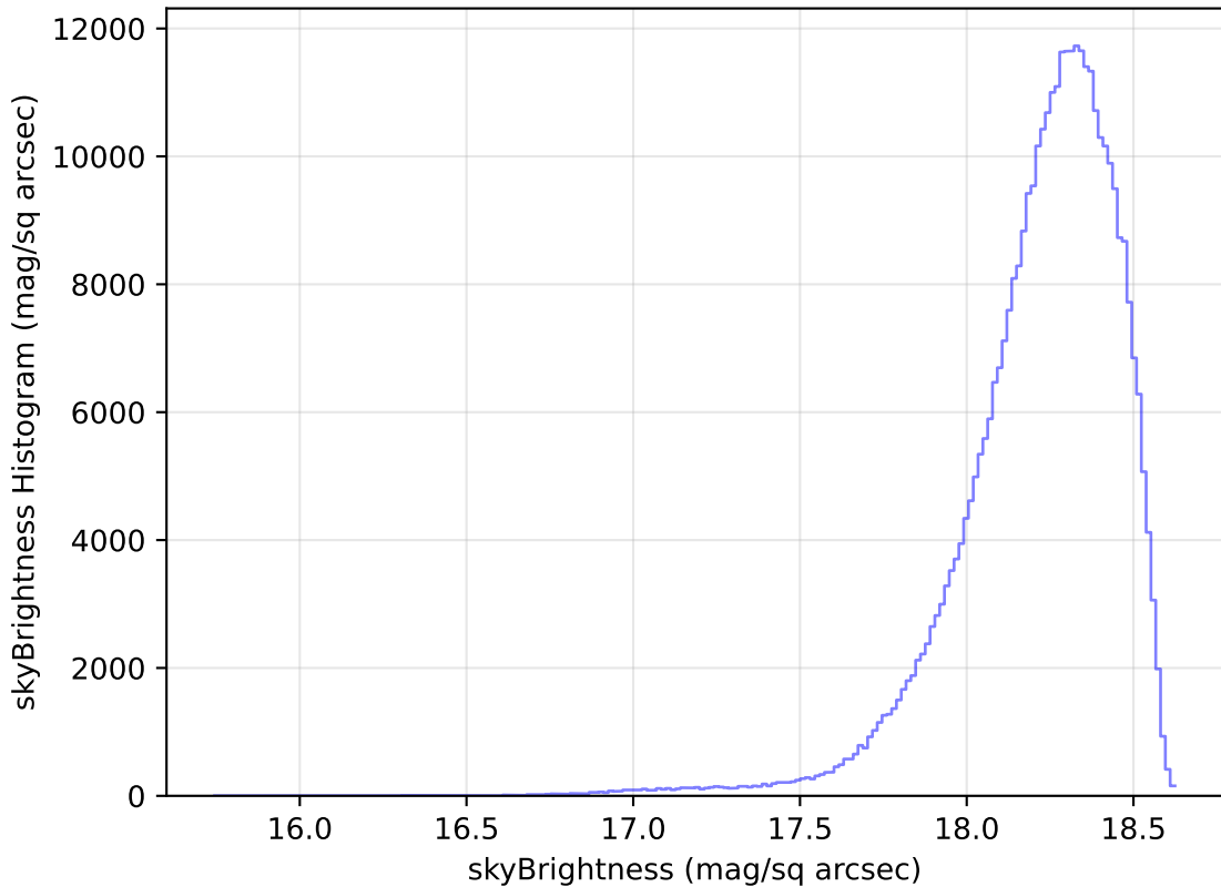
ddf_loaded_half_fl15_v3.4_10yrs WFD y band: skyBrightness Histogram
