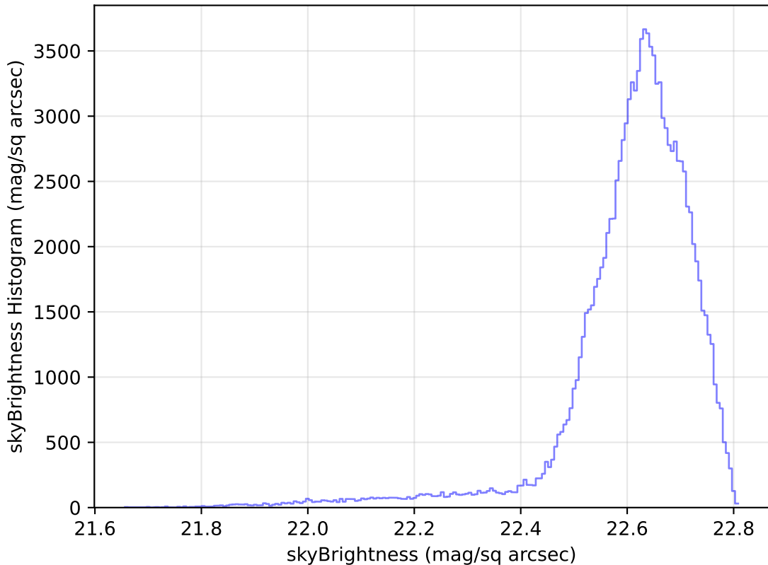
ddf_loaded_half_fl15_v3.4_10yrs WFD u band: skyBrightness Histogram
