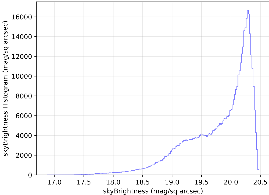
ddf_loaded_half_fl15_v3.4_10yrs WFD i band: skyBrightness Histogram
