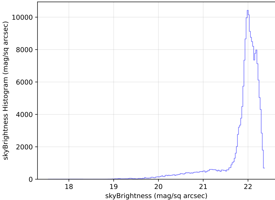
ddf_loaded_half_fl15_v3.4_10yrs WFD g band: skyBrightness Histogram
