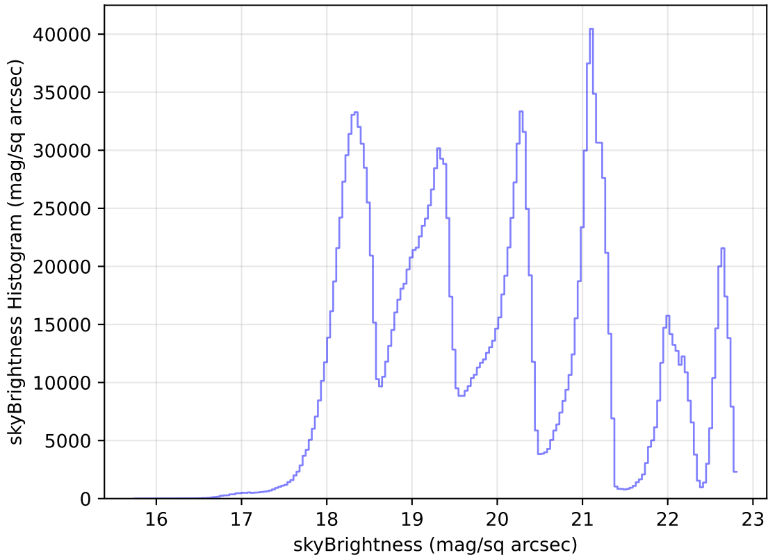
ddf_loaded_half_fl15_v3.4_10yrs WFD all bands: skyBrightness Histogram
