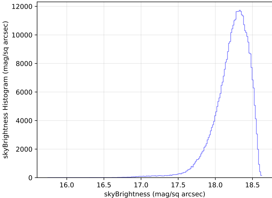
ddf_loaded_half_fl15_v3.4_10yrs All sky y band: skyBrightness Histogram
