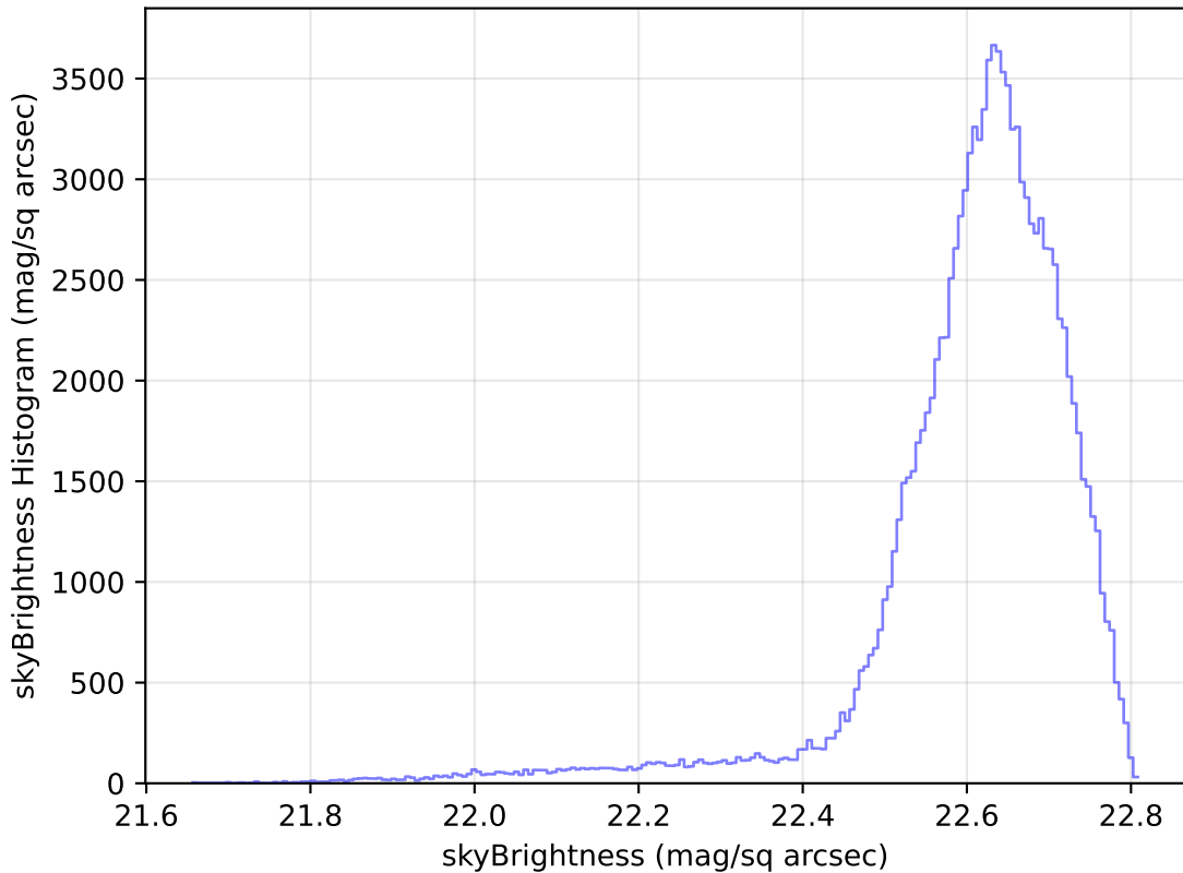
ddf_loaded_half_fl15_v3.4_10yrs All sky u band: skyBrightness Histogram
