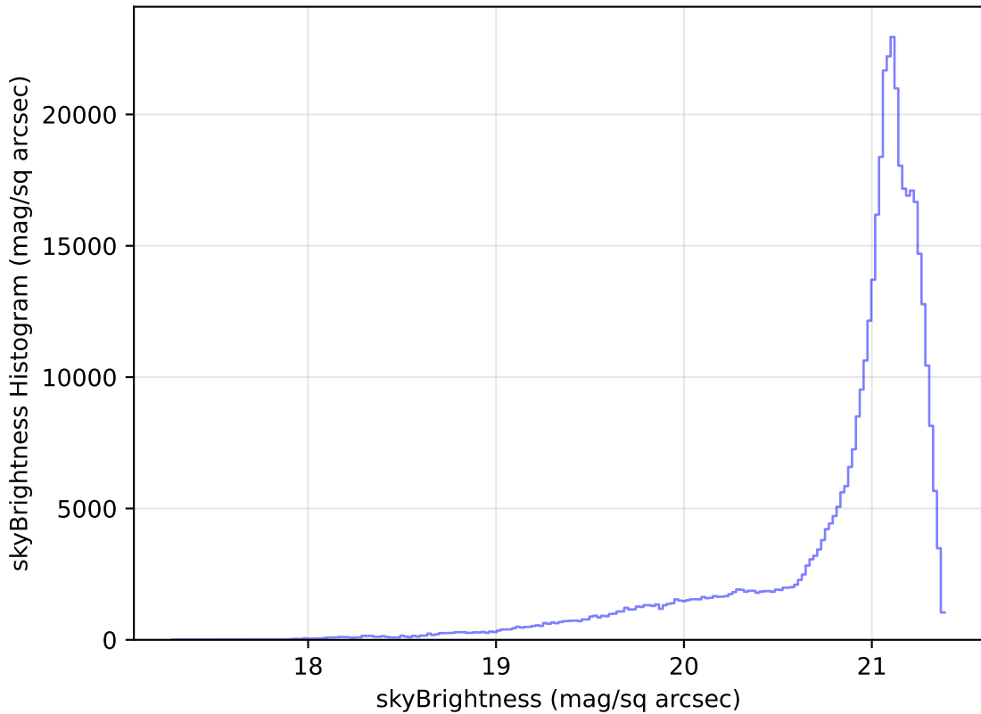
ddf_loaded_half_fl15_v3.4_10yrs All sky r band: skyBrightness Histogram
