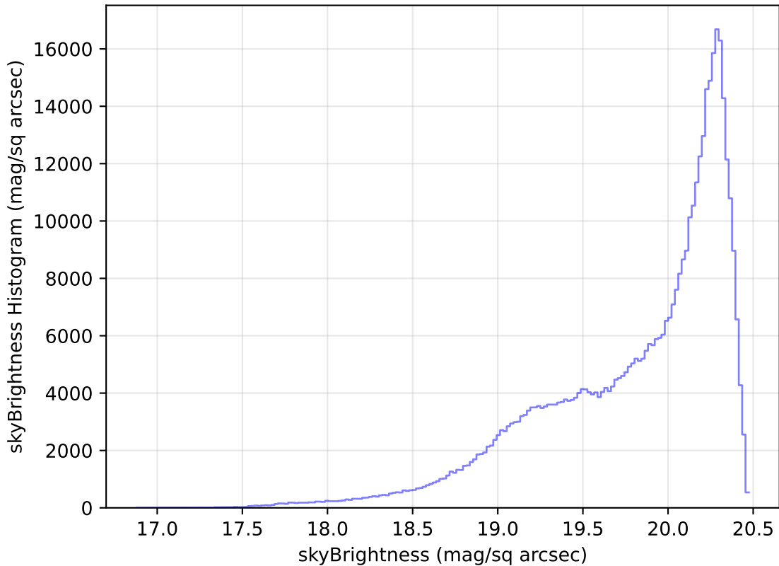
ddf_loaded_half_fl15_v3.4_10yrs All sky i band: skyBrightness Histogram
