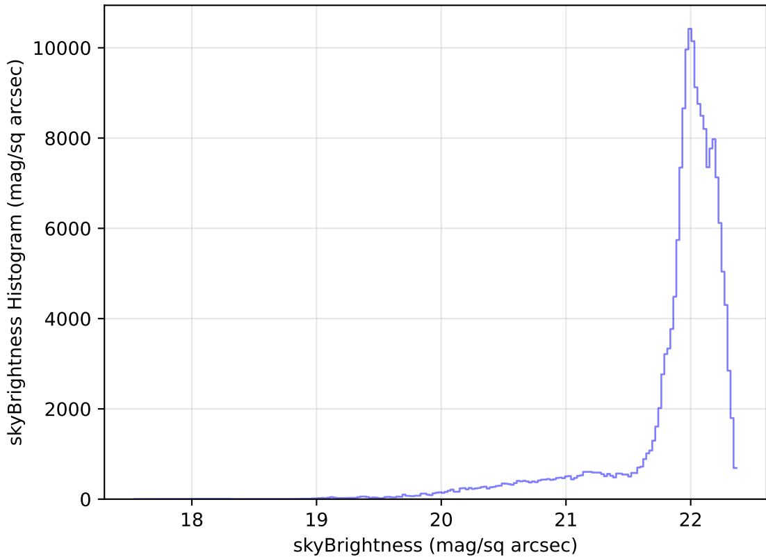
ddf_loaded_half_fl15_v3.4_10yrs All sky g band: skyBrightness Histogram
