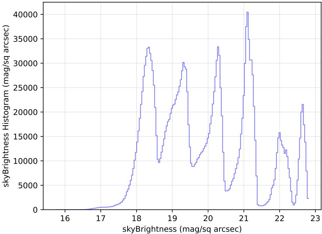
ddf_loaded_half_fl15_v3.4_10yrs All sky all bands: skyBrightness Histogram
