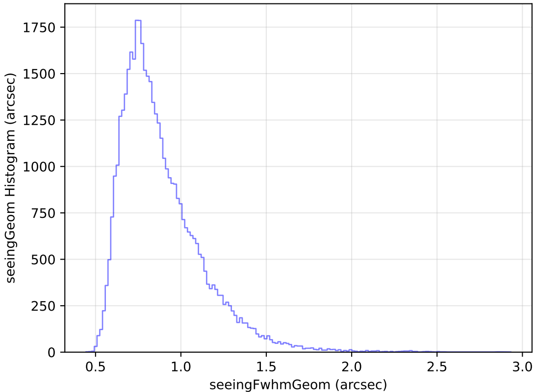
ddf_loaded_half_fl15_v3.4_10yrs Yr 1 z band: seeingGeom Histogram
