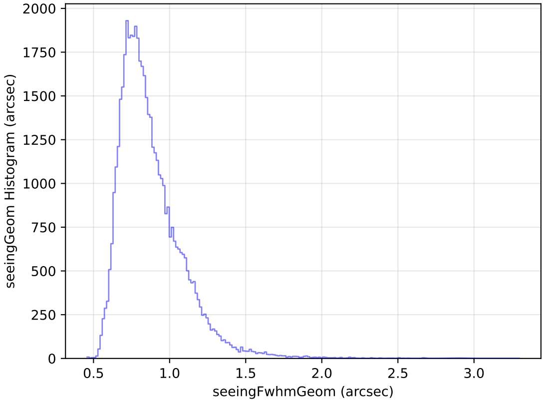
ddf_loaded_half_fl15_v3.4_10yrs Yr 1 y band: seeingGeom Histogram
