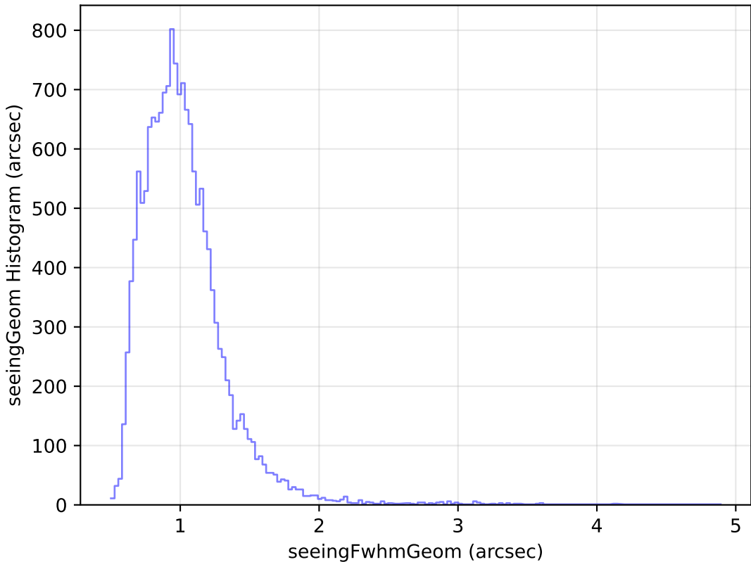
ddf_loaded_half_fl15_v3.4_10yrs Yr 1 u band: seeingGeom Histogram
