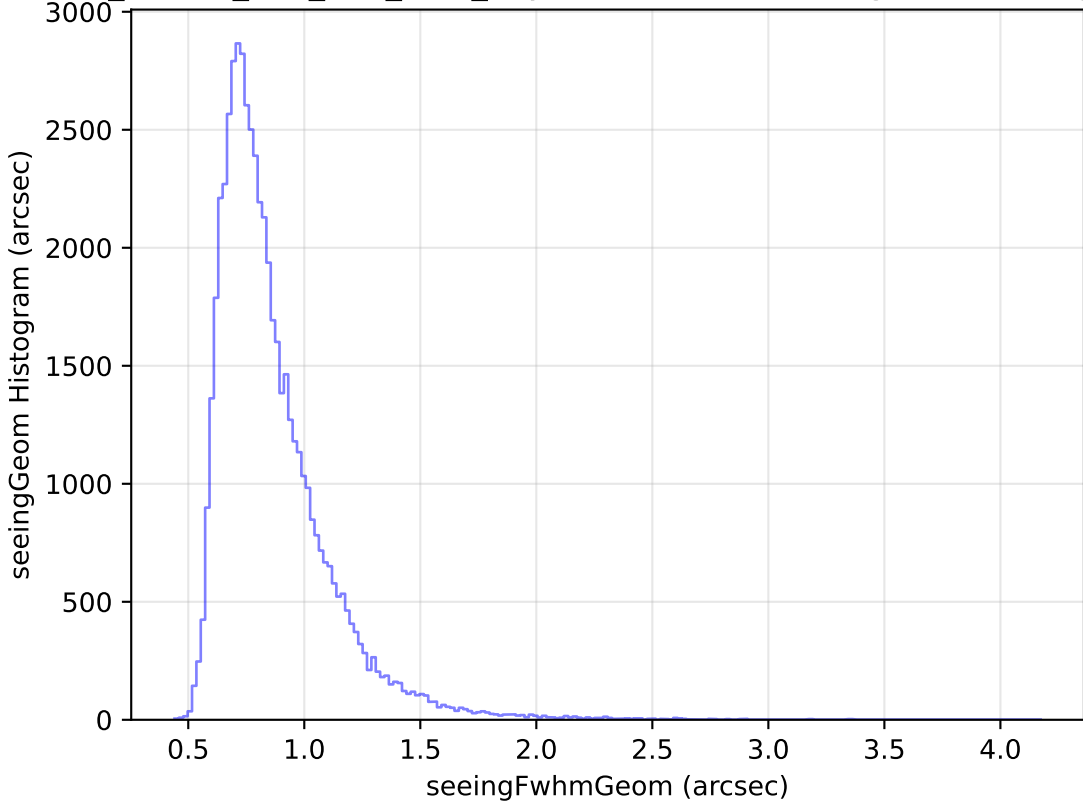
ddf_loaded_half_fl15_v3.4_10yrs Yr 1 i band: seeingGeom Histogram
