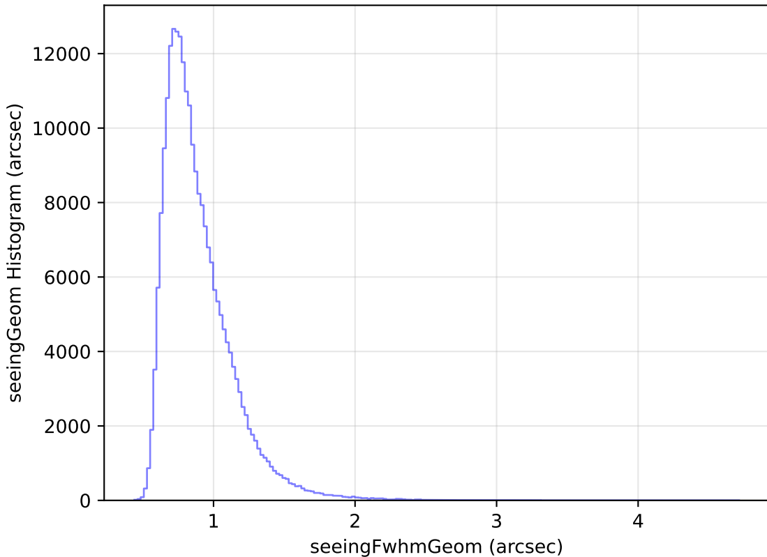
ddf_loaded_half_fl15_v3.4_10yrs Yr 1 all bands: seeingGeom Histogram
