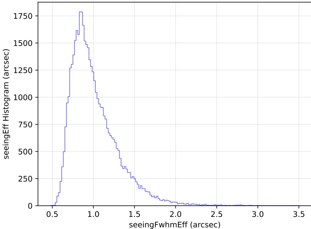
ddf_loaded_half_fl15_v3.4_10yrs Yr 1 z band: seeingEff Histogram
