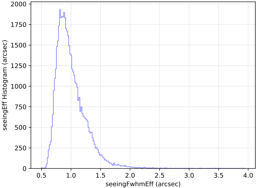
ddf_loaded_half_fl15_v3.4_10yrs Yr 1 y band: seeingEff Histogram
