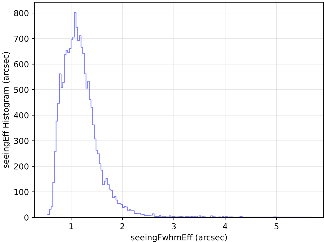
ddf_loaded_half_fl15_v3.4_10yrs Yr 1 u band: seeingEff Histogram
