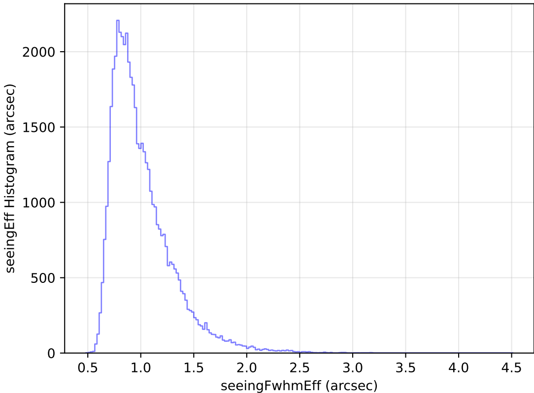
ddf_loaded_half_fl15_v3.4_10yrs Yr 1 r band: seeingEff Histogram
