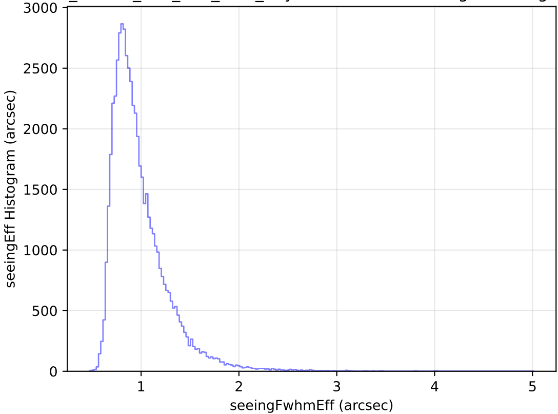
ddf_loaded_half_fl15_v3.4_10yrs Yr 1 i band: seeingEff Histogram
