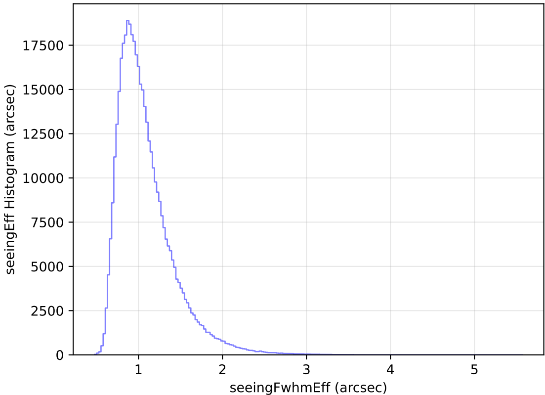
ddf_loaded_half_fl15_v3.4_10yrs WFD z band: seeingEff Histogram
